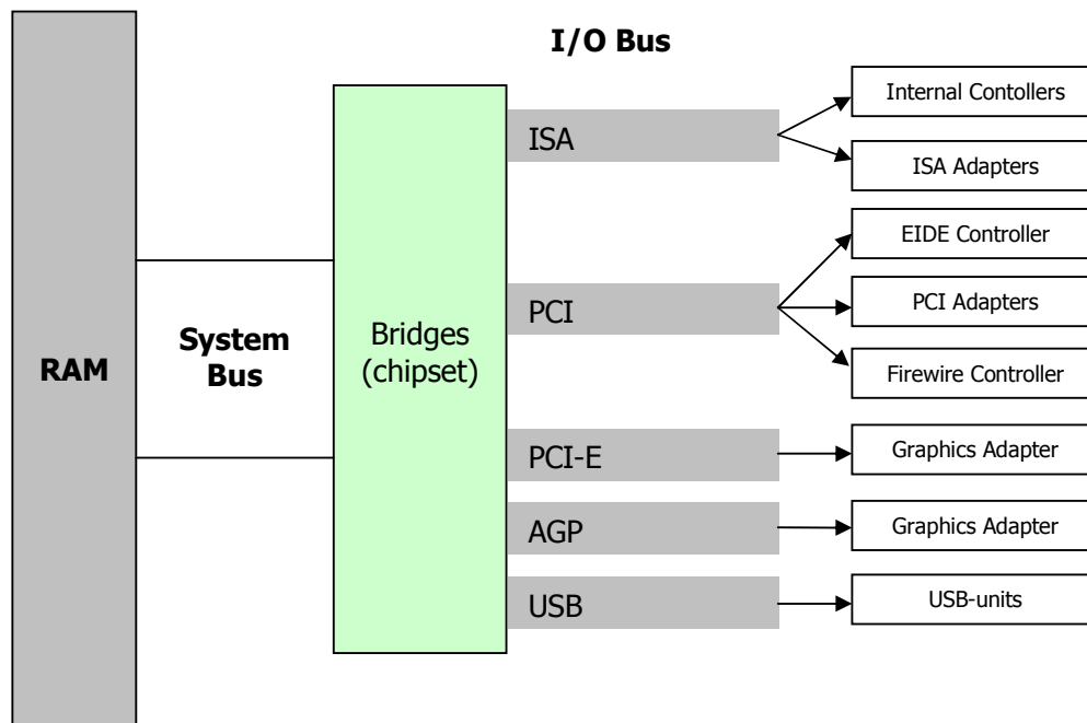
Gambar 5.1 I/O Bus
