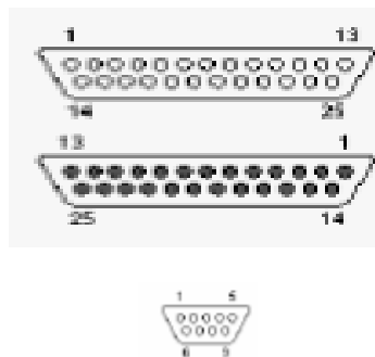
Gambar 5.3 RS-232
