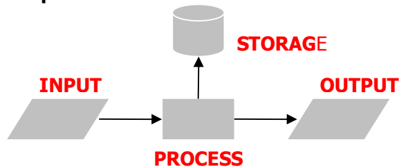
Gambar 2.1 Input-Process-Output Model
